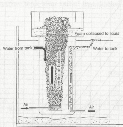
Figure 4: Protein skimmer.
